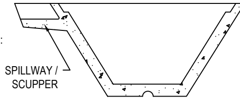
SIDE SECTION
