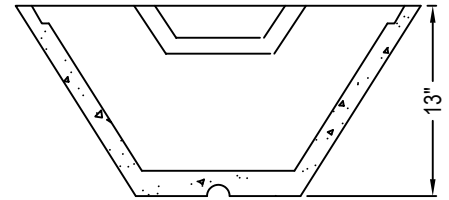
FRONT SECTION
